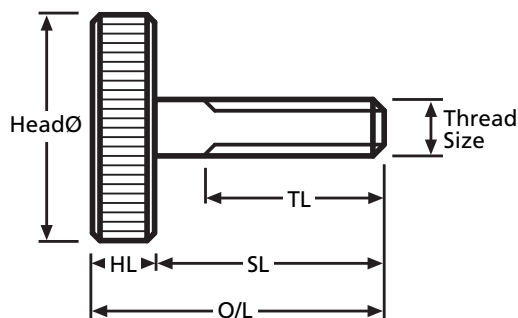
PTS Type
